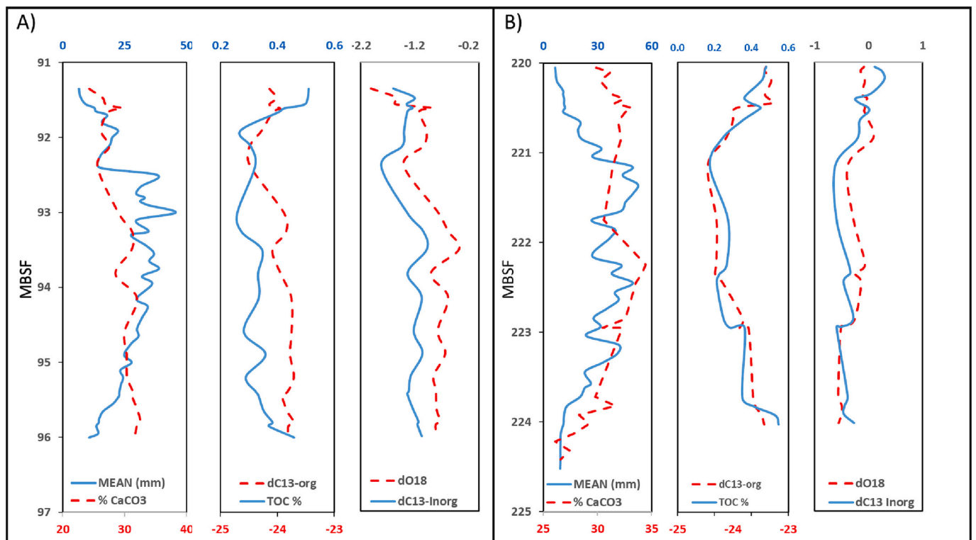
Fig. 16. (A) Distribution of mean grain size, CaCO 3 , TOC, \delta^{13}C_{org} and carbonate oxygen and carbon isotopes through sequence 11H. (B) Distribution of mean grain size, CaCO 3 , TOC, C13-org and inorganic oxygen and carbon isotopes through sequence 25X.
