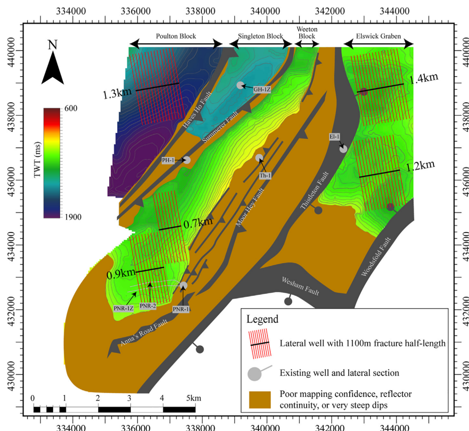
Fig. 16. Map highlighting the areas within the Bowland-12 survey that lateral wells could be employed without hydraulic fractures interfering with major faults or with hydraulic fractures from adjacent wells. The 1100 m predicted half-length of the hydraulic fractures is taken using a proppant cut-off of 1 kg/m 2 . The underlying contour map is the Lower Bowland Shale contoured in two-way time (in milliseconds) (de Jonge-Anderson and Underhill, 2020). The black lines represent the lateral well drilled along minimum horizontal stress orientation and the hydraulic fractures represented as red lines. The brown shading is added where steep dips associated with faulting and folding, or a lack of seismic reflectivity would inhibit drilling.
