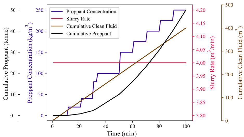
Fig. 5. Illustration of the pumping schedule used for all hydraulic fracture simulations. The schedule was designed based on the planned treatments at well PNR-12 whereby 400 m 3 of fluid and 50 t of proppant were pumped into each completion stage. Proppant concentration ramps from 0 to 250 kg/m 3 with the slurry rate fixed at 4 m 3 /min.
