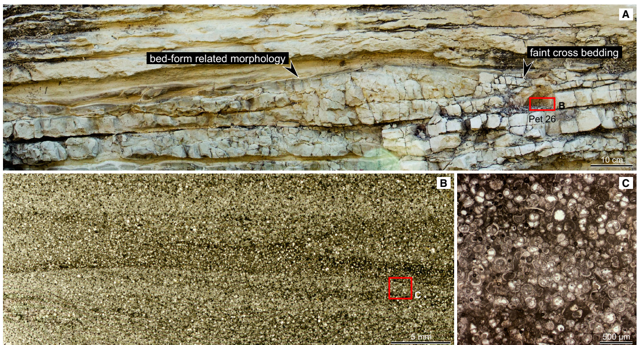
Fig. 15. Calcarenites with internal wavy layering (F3b, globigerinid packstone–grainstone). Interpretation: Calcareous sandy contourite. Early Miocene from the Pakhna Formation as part of Petra Tou Romiou section (Sample Pet 26). (A) Outcrop photograph of a calcarenite bed (F3b) that preserves a bed-form-related upper boundary (mega ripple, subaqueous dune) and relic cross-bedding. (B) Thin-section scan of the calcarenite bed (globigerinid packstone) illustrating local well-preserved cross-lamination (F3b). (C) Microphotograph illustrating the particle-supported texture of the sorted globigerinid packstone (F3b).
