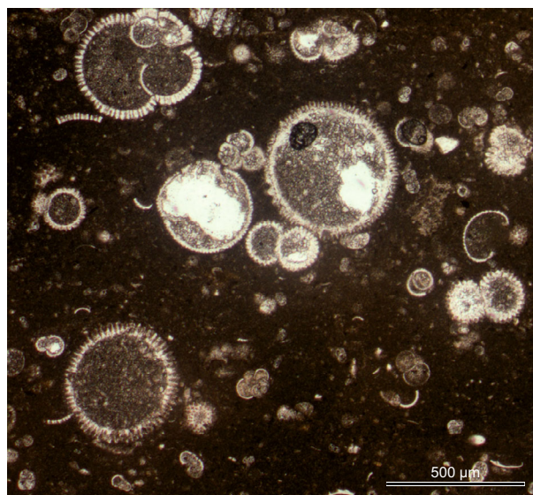
Fig. 17. Microfacies of calcilutites (F2a, globigerinid wackestone), which are interbedded with calcarenites (F3c, globigerinid packstone–grainstone). See Fig. 3 for general lithology. Middle Miocene from the Pakhna Formation (Sample Pet 34). Interpretation: muddy calcareous contourites. Note the differing characteristics (grain size and colour) of the matrix within and around the globigerinid test, which is indicative of reworking and redeposition.
