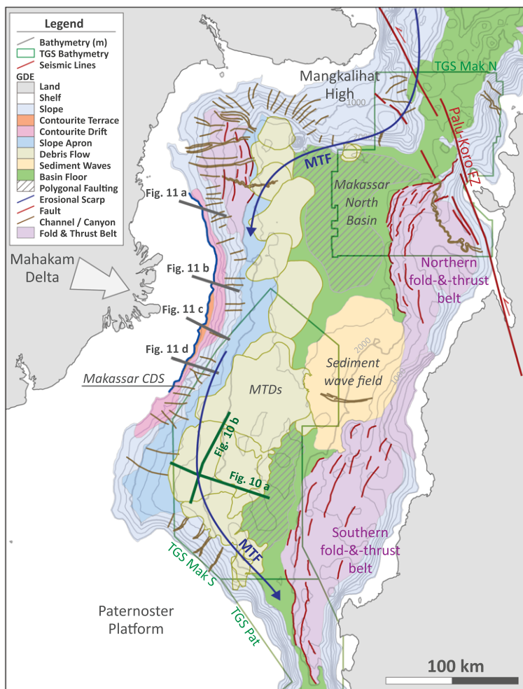
Fig. 12. Map of the environment of deposition of the Makassar North Basin. TGS bathymetry data extent indicates areas of high-resolution data. Additional information gathered from Fowler et al. (2004); Saller and Dharmasamadhi (2012); and Frederik et al. (2019). CDS, contourite depositional system.
