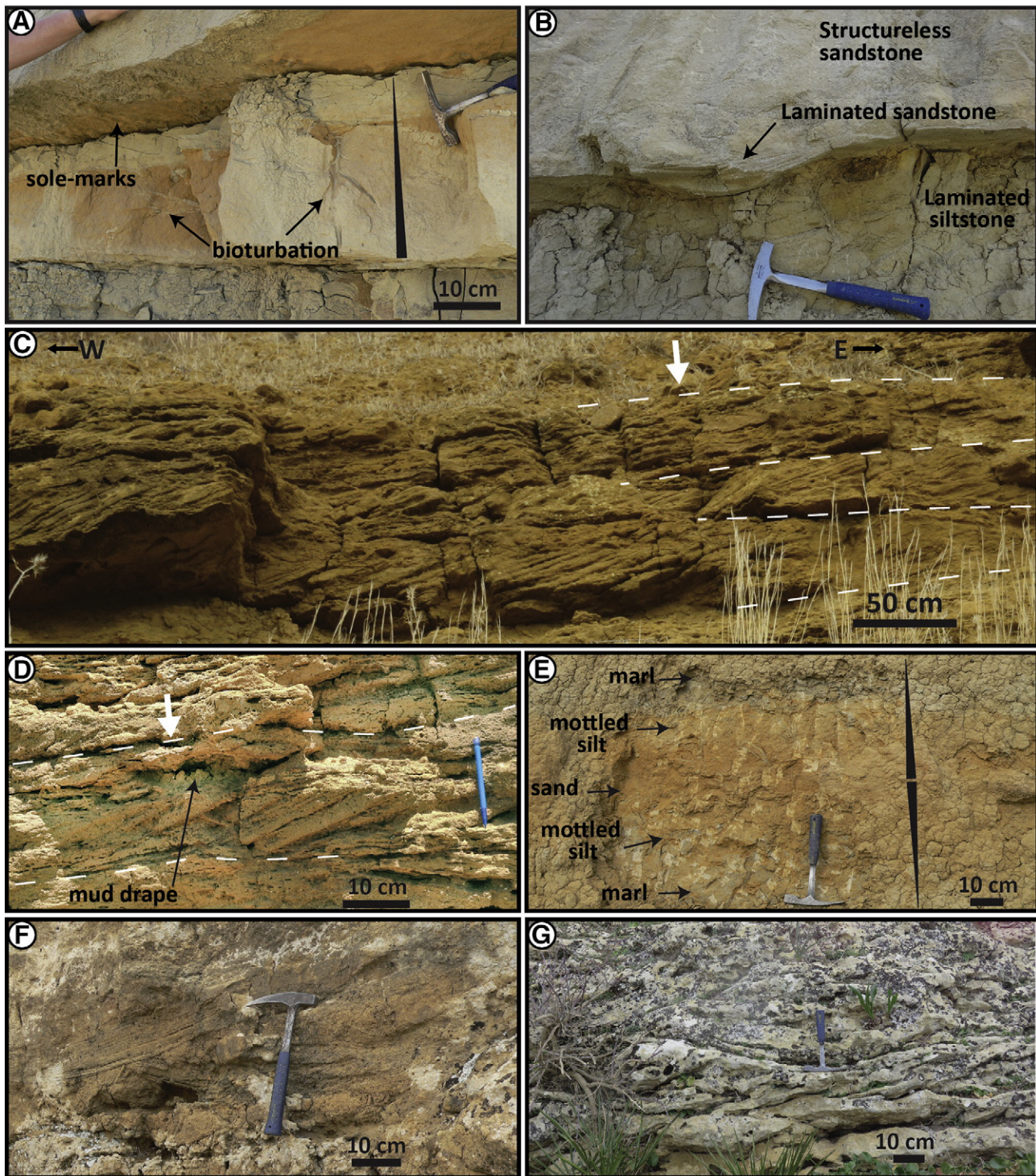
Fig. 6. (A) Close-up of the Sidi Harazem sand-marl alternation, interpreted as sandy turbidites. Bioturbation is interpreted as Zoophycus (left) and Chondrites (right). (B) A sludge-mark at the base of a turbidite bed at Sidi Harazem is filled with a ~5 cm thick cross-laminated sandstone division. (C) 2D cross-sets at El Adergha are mostly unidirectional and up to ~50 cm in thickness. White dotted lines depict surfaces of the clinoforms drawn in Fig. 5D. (D) Small set of cross-bedding and ripple laminations. (E) Close-up observation of a sandy contourite at El Adergha (location in outcrop in Fig. 5D) showing bi-gradational sequences analogous to the contourite facies model of Stow et al. (1998) and Stow and Faugères (2008). (F, G) Examples of the swaley-cross stratification found in the Ain Kansera sandstone intervals.
