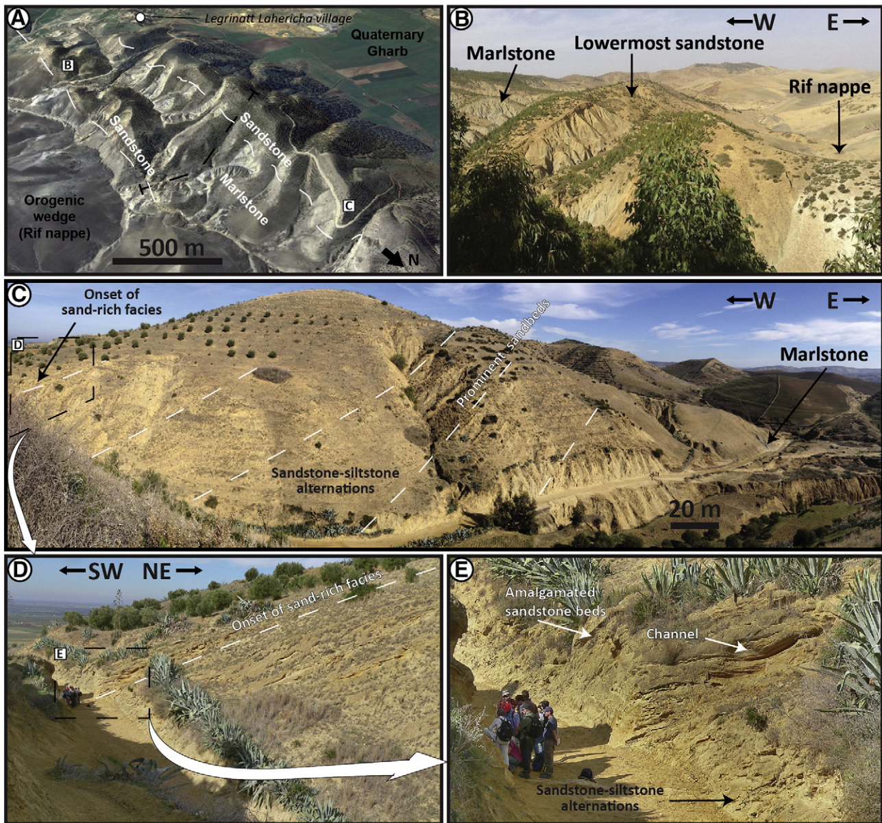
Fig. 13. (A) Oblique satellite image with location of the main lithological units at Mount Haricha. The section is tilted and the layers plunge into the Gharb Basin to the west. Note the view towards the southwest. (B) Panoramic picture showing the contact between the lower part of the section and the Rif nappe of the orogenic wedge. (C) Panoramic picture of the sand-mar alternation of the upper part of the section (white dotted lines are drawn above prominent sand beds). This alternation grades upwards into the sand-rich facies (D). (E) Close-up of the onset of the amalgamated sandstone beds making the top ~50 m of the Haricha section.
