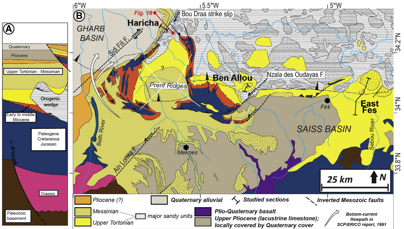
Fig. 2. (A) Stratigraphic column and tectonogram illustrating the relationship between lithostratigraphy and tectonic in the Rif foreland (after Capella et al., 2017). (B) Geological map of the study area with location of the sections (East Fes, Ben Allou, and Haricha) and seismic profile shown in Fig. 16. Tectonic lineaments in the Saiss, eastern Gharb basin, and the southern margin of the external Rif thrust-sheets are compiled after Sani et al. (2007); Capella et al. (2017). The extent of upper Tortonian – Messinian units is modified after the results of the present study.
