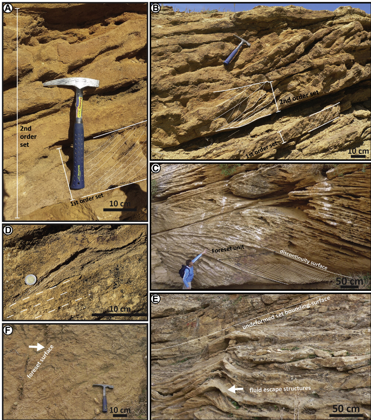
Fig. 9. (A) Relationship between different orders of cross-stratification at Ben Allou. First-order sets are small dunes prograding down the lee-side of larger dunes (2nd order sets). (B) West-migrating, medium thickness, simple cross-bedding with tabular geometry at Ben Allou A, SI-1a. (C) West-migrating, medium to large, compound cross-bedding at Ben Allou B, SI-1a. (D) Well-preserved dune over-riding a larger dune. (E) Fluid-escape structures occur in cross-sets and are capped by undeformed set-boundaries. (F) Planolites burrowing the surface of a foreset.
