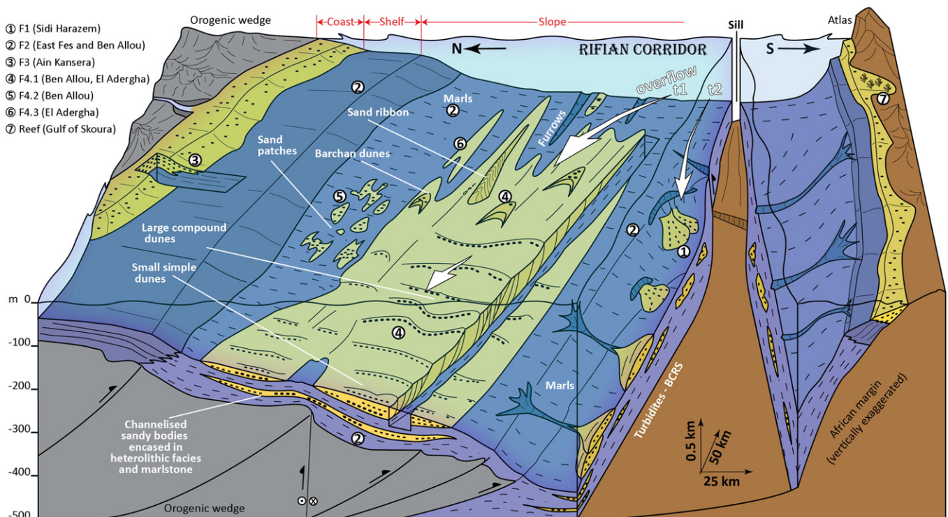
Fig. 17. Interpretative sketch with sedimentary environments and bedform distribution in a deep, foreland-basin seaway. This genetic model relates to a conceptual distribution of bedforms under dominantly unidirectional current and explains the mixed environments observed in the South Rifian Corridor. BCRS = Bottom Current Reworked Sands.
