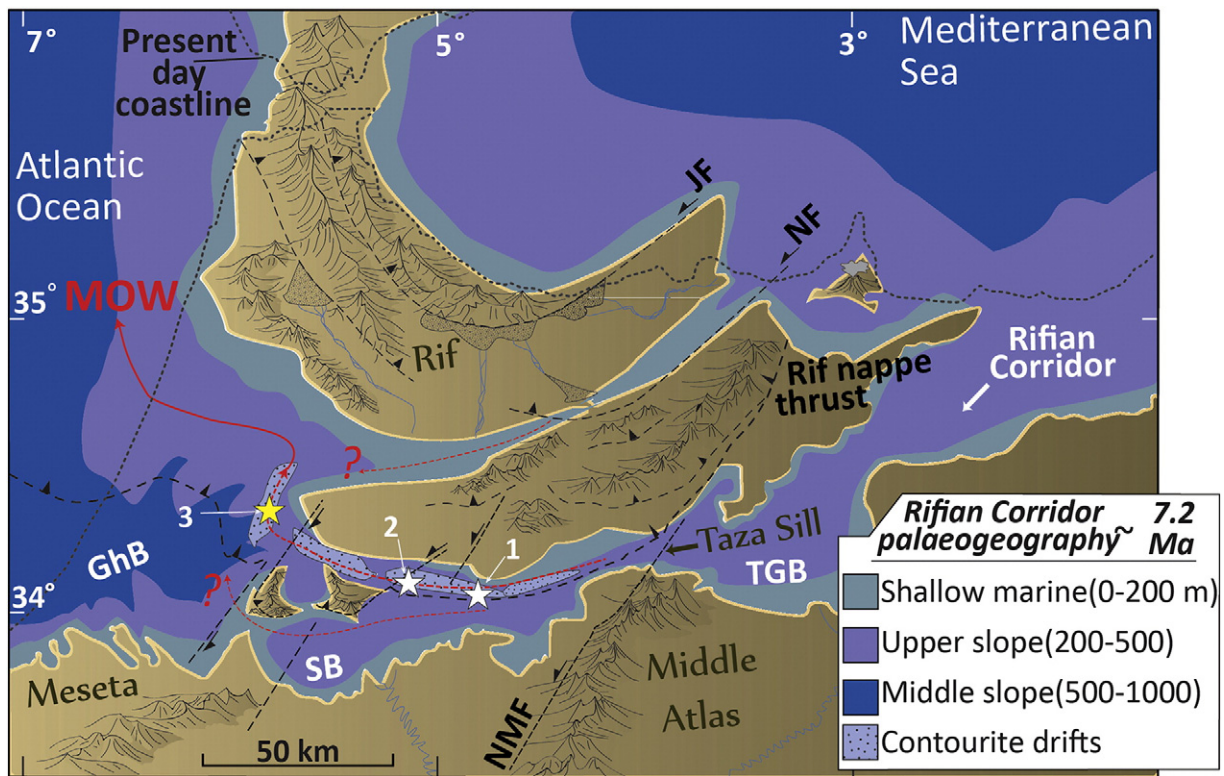
Fig. 18. Palaeogeographic map of the Rifian Corridor at the Tortonian-Messinian boundary. Active tectonic structures after Sani et al., 2007; Chalouan et al., 2014; Capella et al., 2017. NF: Nekor Fault; JF: Jebha Fault; NMF: North Middle-Atlas Fault. GhB: Gharb Basin; SB: Saiss Basin; TGB: Taza-Guercif Basin. Sections indicated with a white star are: El Adergha (1), Ben Allou (2). Yellow star depicts the position of the drift inferred from seismic data in the Gharb Basin (Fig. 16).
