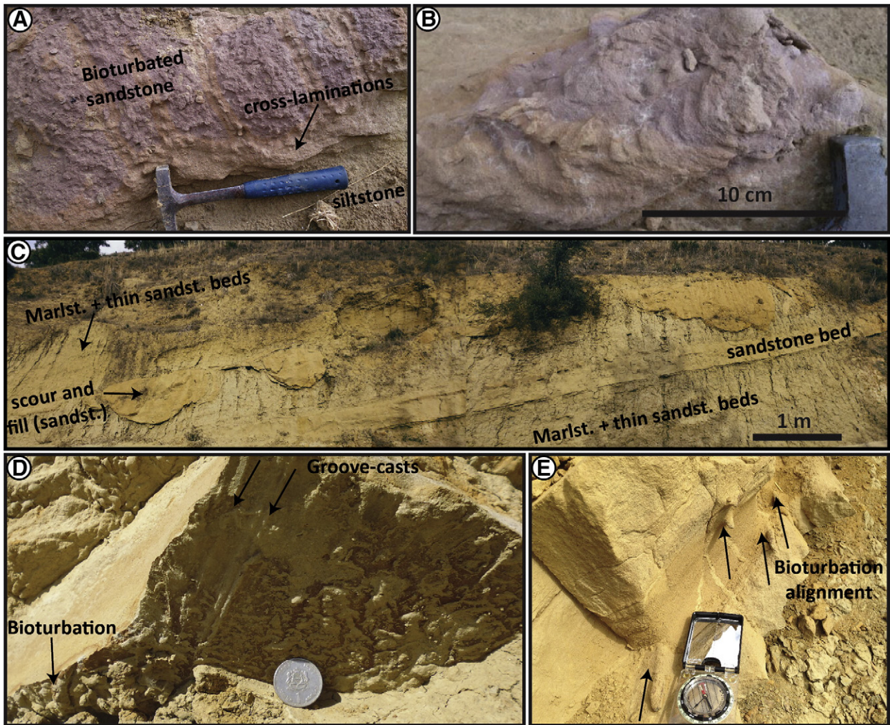
Fig. 14. Close-ups on turbidite features at Haricha. (A) Purple-coloured sandstone bed from the lower part, with a basal division of cross-lamination. Note the bioturbation throughout. (B) Bioturbation on the top of the same sandstone beds, interpreted as Rhizocorallium . (C) Photomosaic of a road cut showing tabular sandstone beds and sandstone with scour-and-fill features. The sandstone beds are encased in silty marlstones. (D) Sole-marks (groove-casts) in a bioturbated base. (E) Example of a sand bed with superposition of divisions of massive sand (base) and parallel-laminated sand. Preferential orientation of bioturbation-like features is shown.
