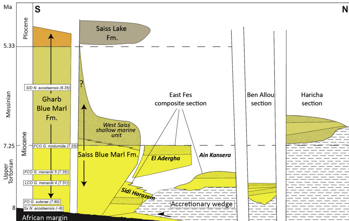
Fig. 3. Correlation diagram between the studied sections and the classic Gharb-Saïss stratigraphy. The 5 studied sections (Sidi Harazem, El Adergha, Ain Kansera, Ben Allou, and Haricha) are dated with biostratigraphy. Bioevents (left column): Sx = onset dominant sinistral; FO = first occurrence; LCO = last common occurrence; FCO = first common occurrence; S/D = coiling change from predominantly sinistral to dextral (after Lourens et al., 2004; Hilgen et al., 2012). Dotted fills depict the sand-rich parts, whereas simple colour fill broadly represents other lithologies (e.g., marlstone, limestone).
