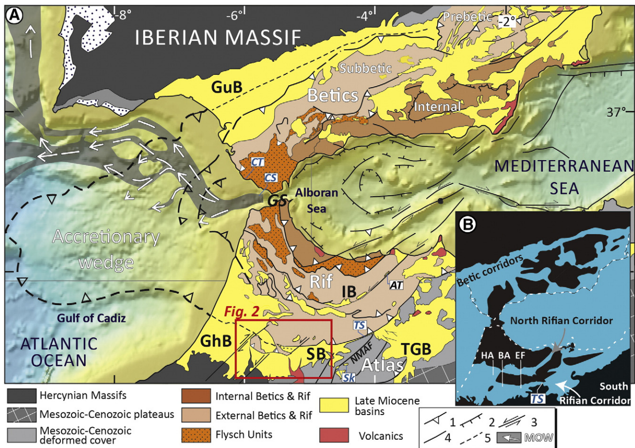
Fig. 1. (A) Generalised tectonic map of the Betic-Rif arc with location of the study area (Fig. 2) and distribution of the Mediterranean Overflow Water. Structural units modified after Vergés and Fernández (2012). AT: Arbaa Taourirt; CS: Camarinal Sill; CT: Cape Trafalgar; GhB: Gharb Basin; GS: Gibraltar Straits; GuB: Guadalquivir Basin; IB: Intramontane Basins; NMAF: North-Middle-Atlas Fault; SB: Saiss Basin; Sk: Gulf of Skoura; TGB: Taza-Guercif Basin; TS: Taza Sill. 1: thrust; 2: normal fault; 3: strike-slip; 4: faults; 5: buried thrust. (B) Approximate palaeogeography of the Betic and Rifian Corridor during the late Miocene modified after Flecker et al. (2015). White dotted lines are the present-day coastline. Location of the studied section in the palaeogeographic context: BA = Ben Allou; EF = East Fes; HA = Haricha.
