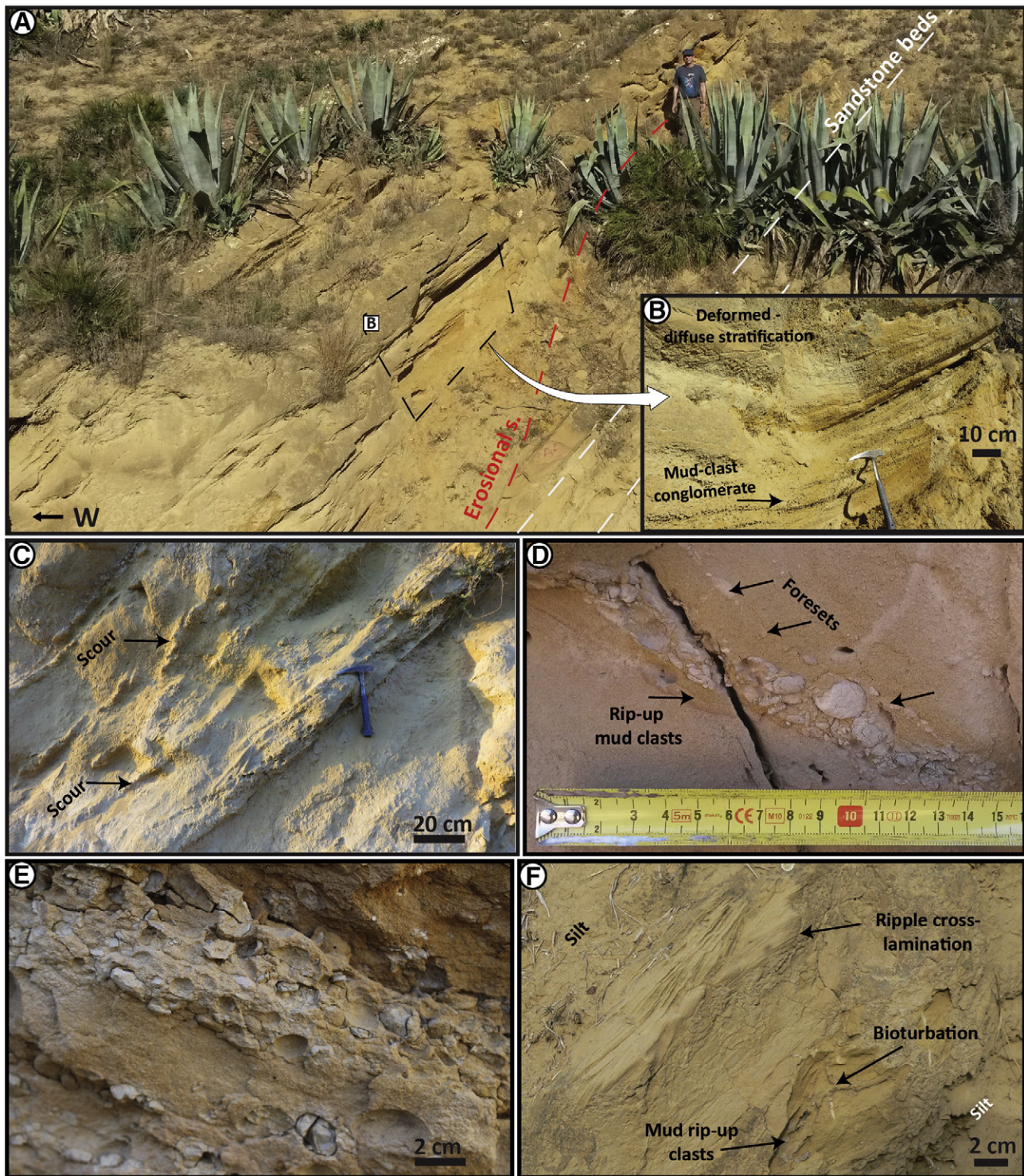
Fig. 15. Details of Haricha-top sand-rich facies, interpreted as deep-water massive sands. (A) Outcrop view of the base of the ~50 m thick, sand-rich facies. White dotted lines depict the bedding attitude of the underlying turbidite beds. (B) Close-up of the mud-clast conglomerate forming scours and diffuse (or deformed) stratification in the amalgamated beds. (C) Scours in coarser layer. (D) Rip-up mud clasts occur between massive sand (below) and cross-laminated sand (above). (E) Example of chaotic mud clast conglomerate. (F) Close-up of a thin (20 cm thick) sandstone bed encased in ungraded siltstone.
