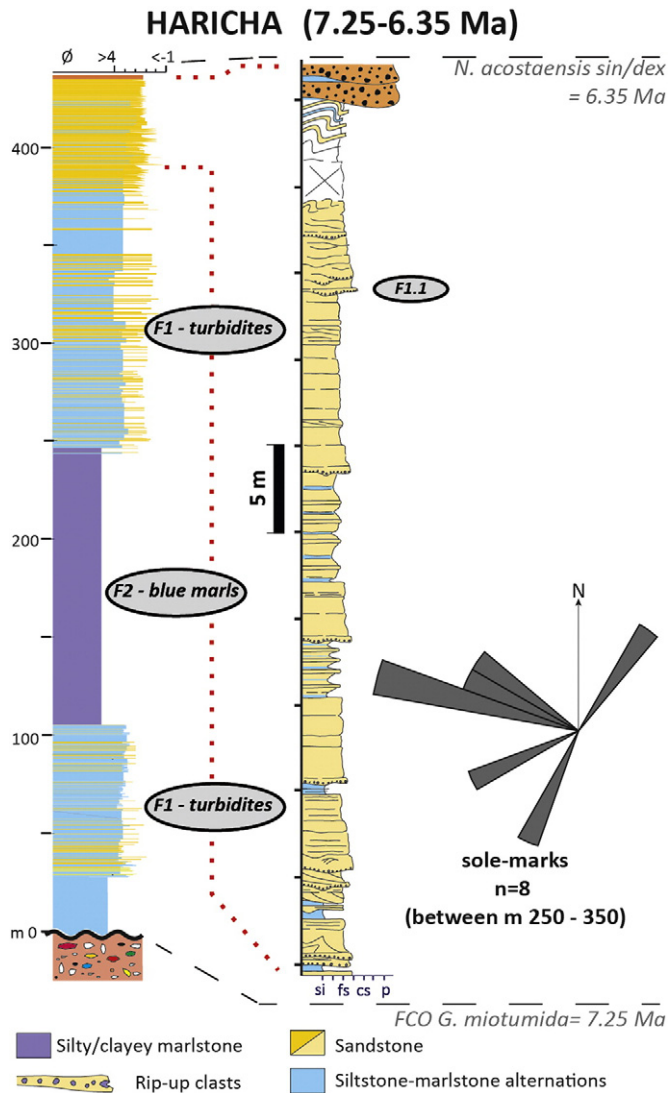
Fig. 12. Stratigraphic log of the Haricha section, with detailed sedimentary log of the top ~50 m, sand-rich facies. Plotted palaeocurrent data corresponding to sole-marks in the sand-marl alternations.
