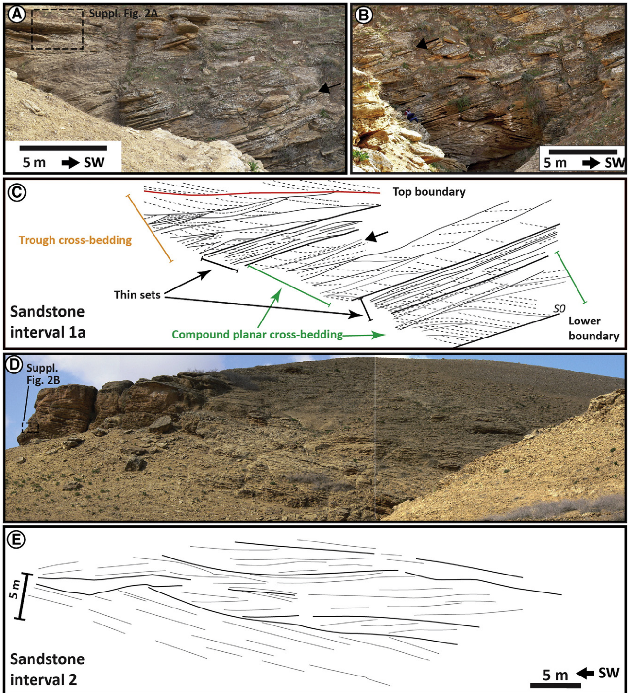
Fig. 10. (A–B) Photomosaic showing the lowermost cross-stratified succession at Ben Allou B, truncated by the channel-form of Fig. 8C at the top. The first set on the right corresponds to Fig. 9C. The black arrow indicates the same bed. (C) Line drawing of the combined pictures A–B. (D) Photomosaic of a cross-stratified succession in SI-2. For location see Fig. 8E. (E) Line-drawing of (D) with emphasis on the discontinuities between sets.
