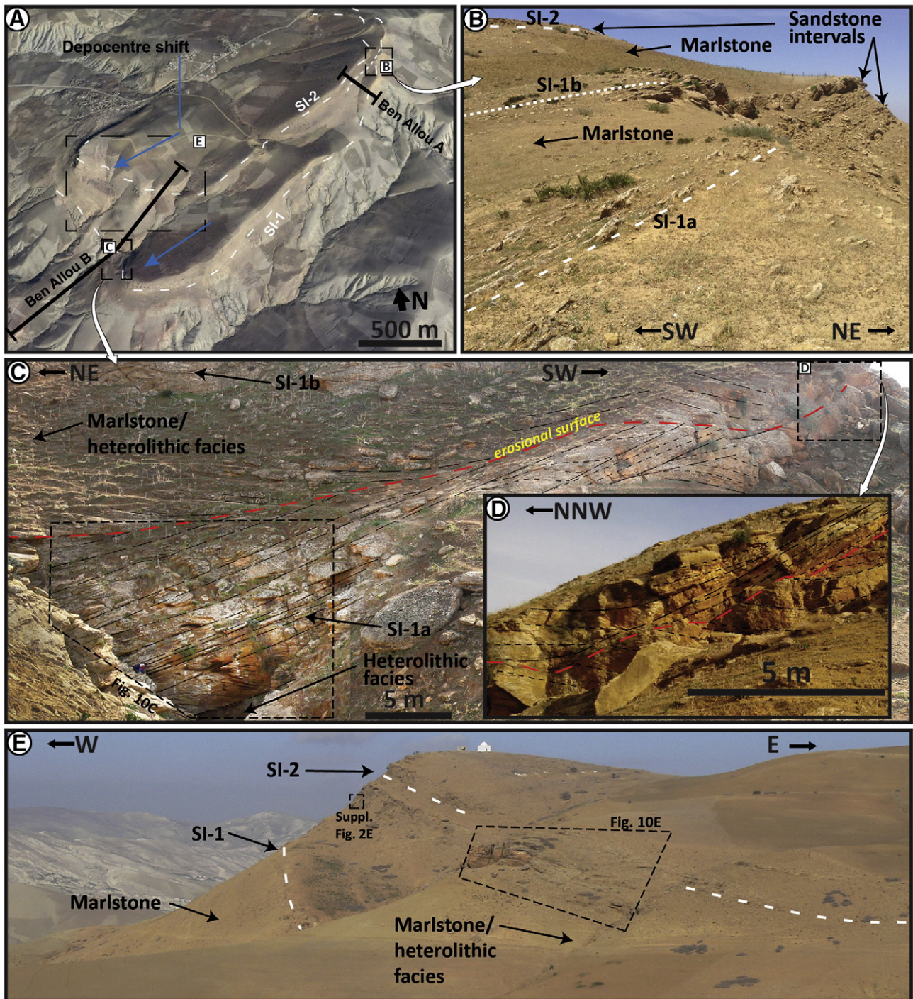
Fig. 8. (A) Oblique satellite image of the Ben Allou section with location of the logging paths (Ben Allou A and B), linear trend of sandstone intervals 1 and 2, and pictures B, C and E. (B) Outcrop view of Ben Allou A section. There is a discordance (angular unconformity) between SI-1a and SI-1b. The marlstones between the two units are wedging out towards the northeast. (C) Sandstone interval 1a at Ben Allou B showing the lateral continuity of the cross-sets, and channel-form displaying an ENE-WSW axis, a width of around 50 m and incision depth of 15 m. (D) Side-view of the same channel-form of C with view to the north-east. (E) Panoramic view of the discordance between sandstone intervals 1 and 2 at Ben Allou B. The two intervals bend in a gentle synform.
