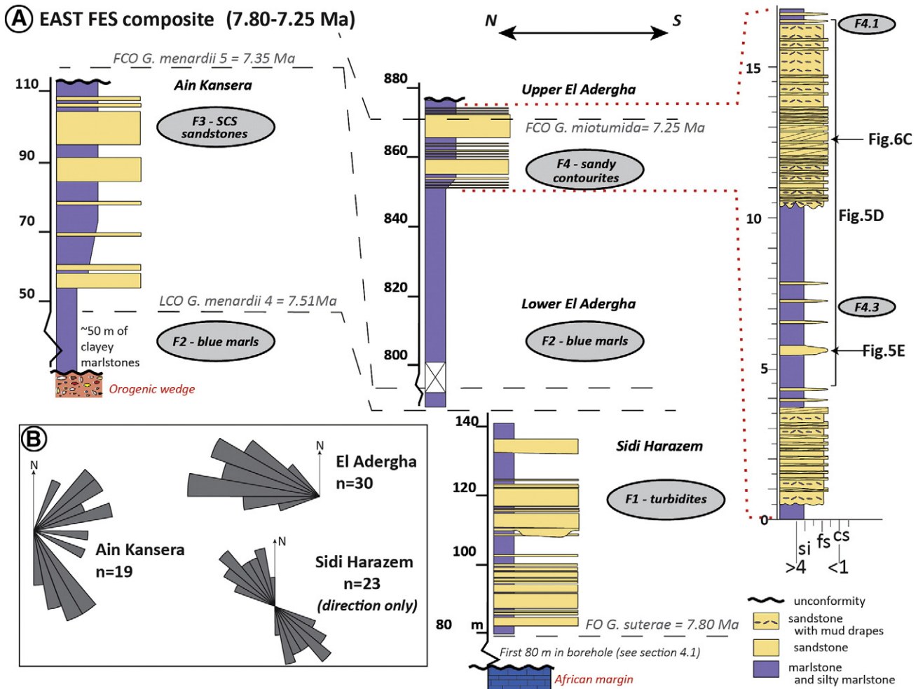
Fig. 4. (A) Stratigraphic logs of Sidi Harazem, El Adergha and Ain Kansera units with brief lithological description and age determination based on planktonic foraminifera (see text for further details). Detailed sedimentary log of the upper part of El Adergha shows the stacking pattern of the cross-stratified sand beds. Location of the sites on Fig. 5A. (B) Palaeocurrents from the three units showing number (n) of data per each site.
