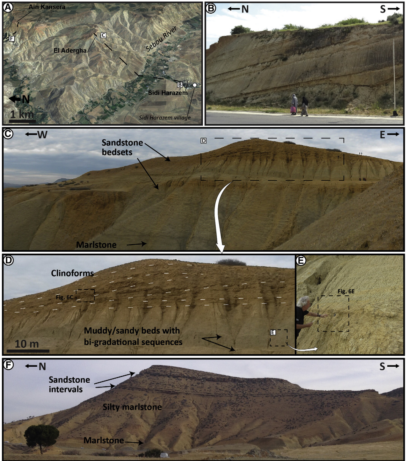
Fig. 5. (A) Satellite image of the East Fes section, showing the location of the Sidi Harazem, El Adergha, and Ain Kansera units, and of pictures B, C, and F (adapted from Google Earth). (B) Outcrop of the Sidi Harazem section, showing the typical sandstone-marlstone alternation. (C) View of the El Adergha section. (D) Close view of the upper El Adergha section, showing the geometry of the upper bedset with prograding clinoforms. (E) Example of one of the sandstone–mudstone beds with bi-gradational sequences from El Adergha, interpreted as contourites. (F) Outcrop view of the Ain Kansera section, showing laterally extensive sandstone intervals at the top.
