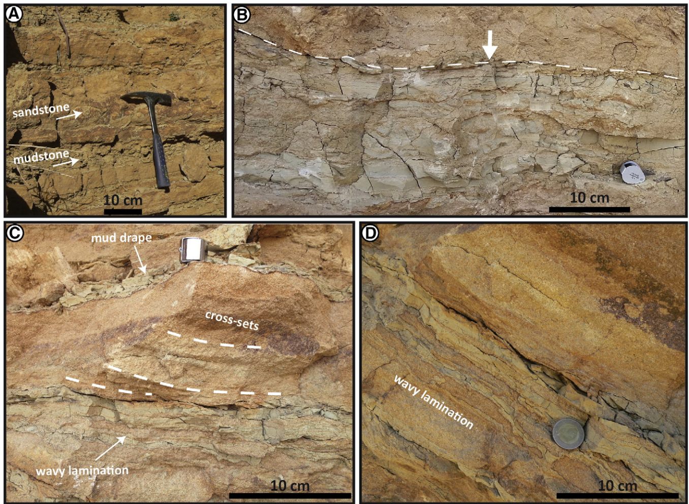
Fig. 11. (A) Heterolithic beds composed of cm- to dm-thick sandstone intervals and mm- to cm-thick mudstone layers. (B) Wavy bounding surface between mudstone layers and sandstone beds. In the top right corner, indistinct cross-laminations are visible. (C) Small cross-sets are preserved in some of the sandstone beds. Note the mudstone draping the bedform geometry. (D) Wavy lamination formed by thin alternations of mudstone and sandstone.
