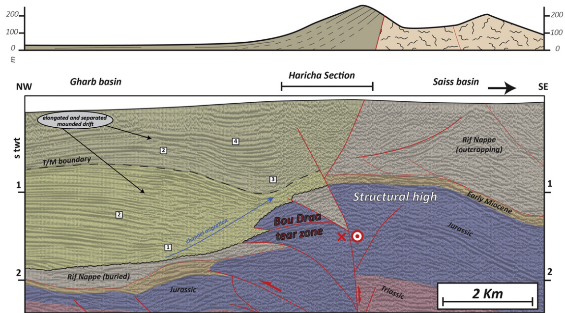
Fig. 16. ONHYM (Office National des Hydrocarbures et des Mines) multichannel seismic line (below) crossing the Haricha section and prolongation of structures to the surface (above). Profile location in Fig. 2. The profile shows the Tortonio-Messinian, post-orogenic (post-nappe) seismo-stratigraphic units with an elongated, separated mounded drift. Seismic facies: (2) continuous and sub-parallel reflections; (1) discontinuous, sigmoidal, and downlapping reflections; (3) channel or moat; (blue arrow) channel migration.
