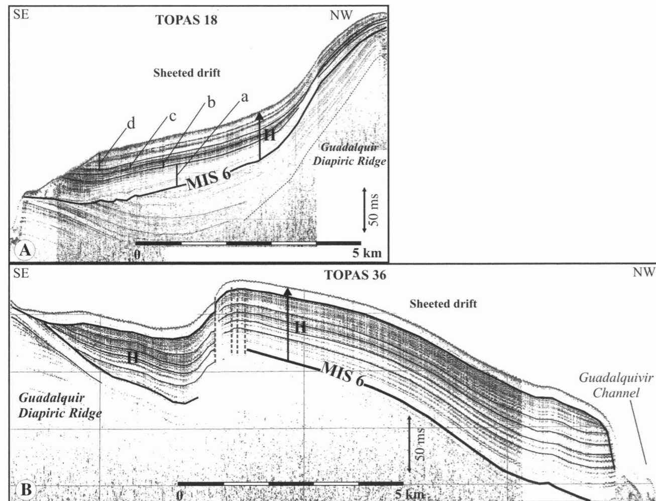
Fig. 6 (a) Ultra high resolution seismic profile showing the minor seismic units within the H sequence of the eastern area of the central sector of the middle slope (modified from Llave et al. 2007); (b) Ultra
