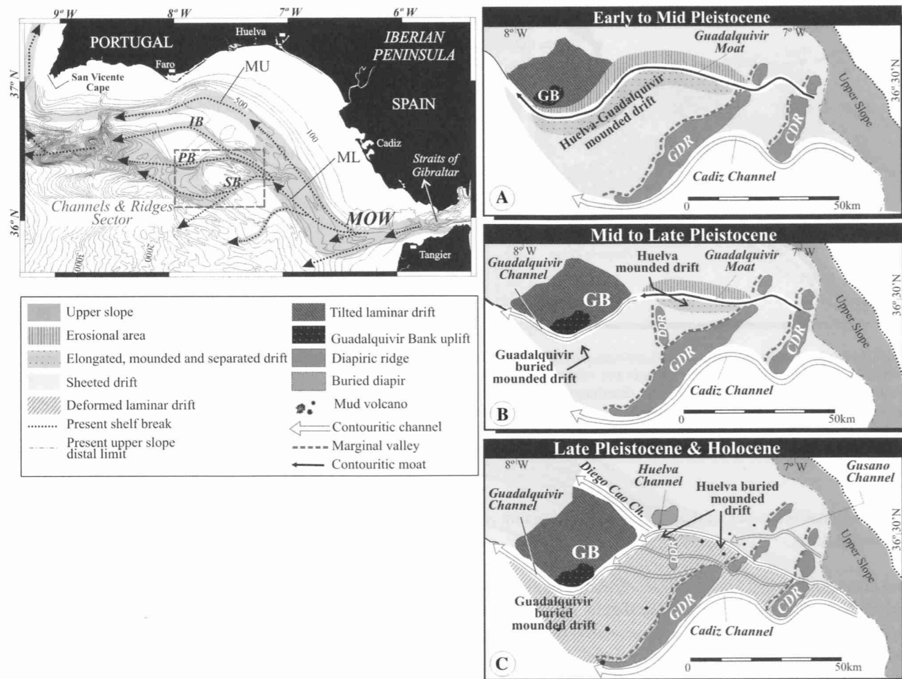
Fig. 8 Interpretative sketch of the Quaternary evolution of the buried mounded drift deposits in the Channels and Ridges Sector of the middle slope of the Gulf of Cadiz. Three different stages have been identified: (a) active Guadalquivir and Huelva drift growth stage (Early to Mid Pleistocene); (b) late-stage drift growth (Middle-Late Pleistocene) and (c) complete drift burial (Late Pleistocene and
