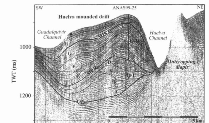
Fig. 5 High resolution sparker seismic profile through part of the Huelva buried mounded drift (HBD) of the central sector of the middle slope (see Fig. 1b for location). Main tectonic and stratigraphy discontinuities are shown
