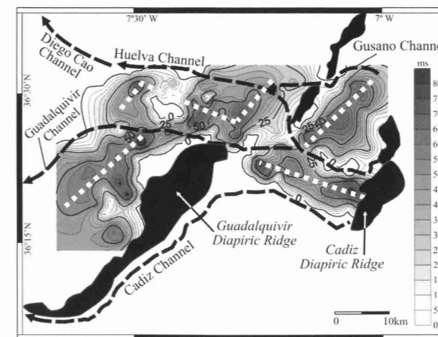
Fig. 7 Isopach map in milliseconds of seismic unit H above the Huelva buried mounded drift in the channels and ridges sector of the middle slope of the Gulf of Cadiz. The distribution of the main depocenters is showed (white dot line), and the present situation of the main contourite channels (black dash lines) and diapiric ridges (solid black), with a NNE–SSW direction is represented
