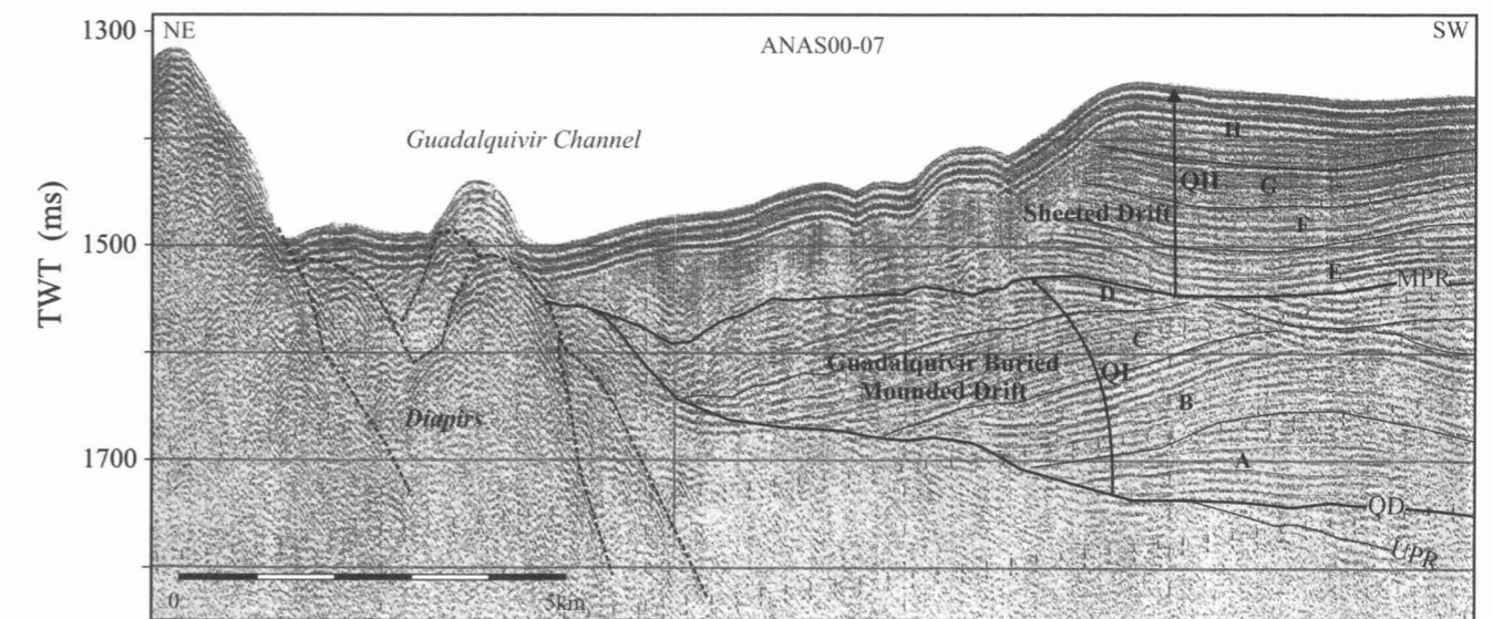
Fig. 3 Sparker seismic profile through part of the Guadalquivir buried mounded drift (GBD) of the western area of the central sector of the middle slope (see Fig. 1b for location). UPR, QD and MPR
