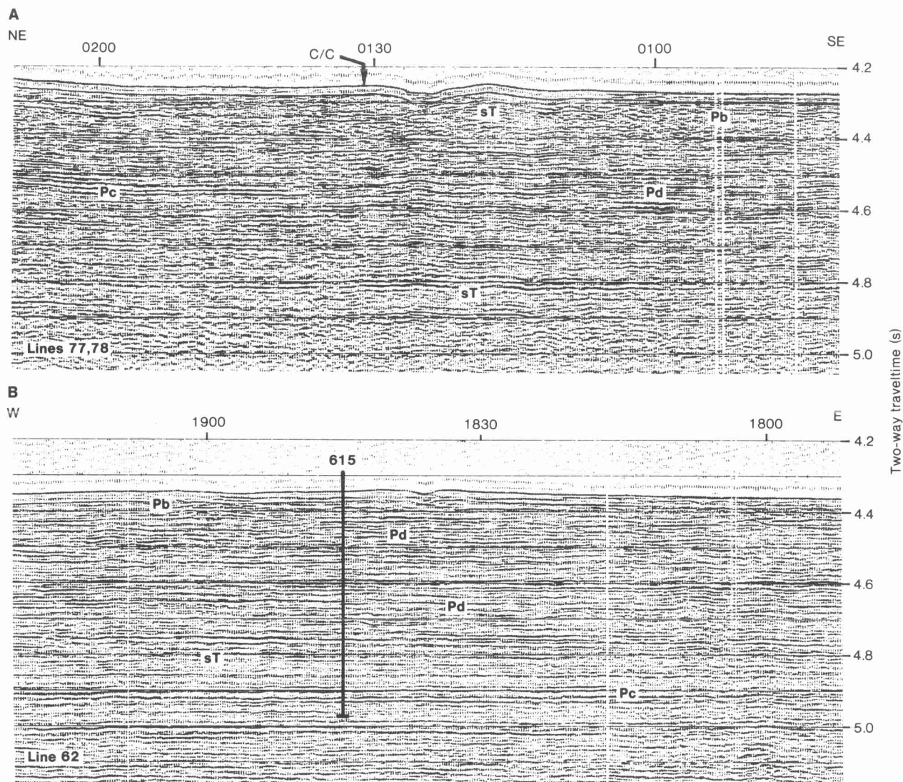
Figure 12. High-resolution (80 cu. in. water gun) seismic profiles and corresponding line drawings showing characteristics of lower-fan channel. Lines (R/V Conrad ) identified on seismic profiles. Bold line ("paleobathymetry") on line drawing (A) at about 4.4 s denotes possible depositional lobes. See Figure 4 for location; Table 1 for seismic facies symbols. C/C = course change.
