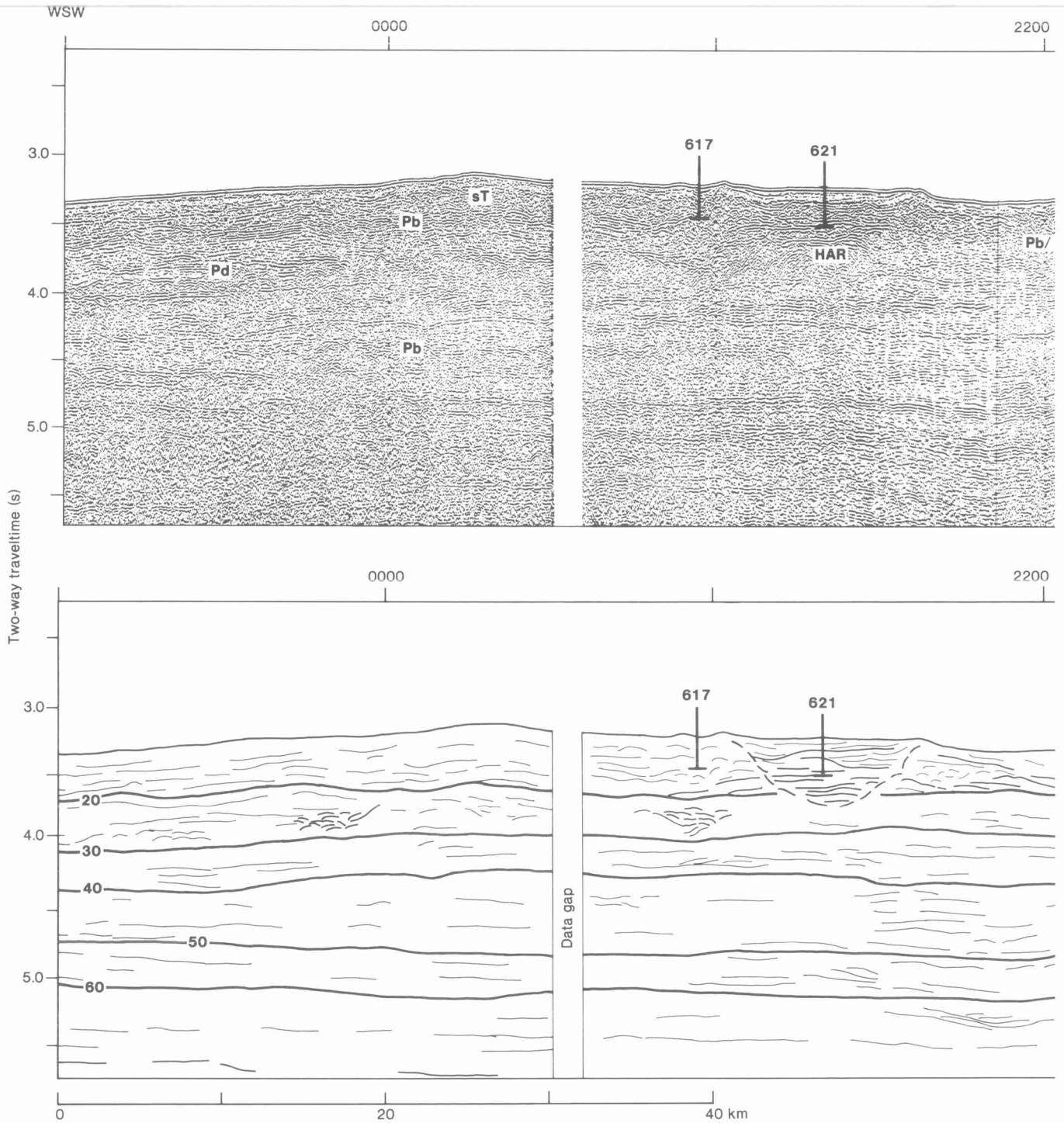
Figure 8. Sparker (160 kJ) seismic profile and line drawing across middle fan showing seismic characteristics and cross-sectional profiles of five fan lobes (U.S.N.S. Kane , Line KB-7). Tentative ages of major horizons listed in Bouma, Coleman, and Meyer (this volume). Extrapolation of Horizon 20 through "slump" area based on drilling results at Sites 616 and 620. Relative positions of Sites 617, 620, and 621 projected onto profile and drawing. See Figure 4 for location; Table 1 for seismic facies symbols.
