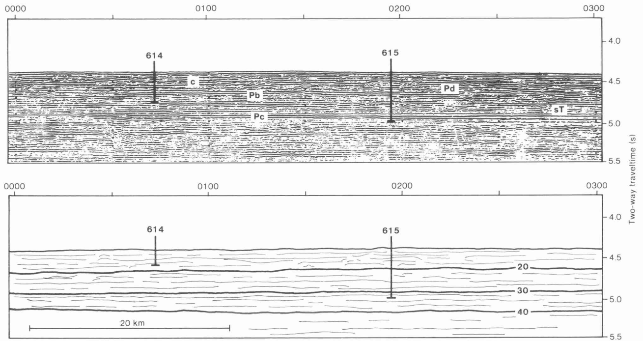
Figure 11. Sparker (160 kJ) seismic profile and line drawing over "distal" portion of lower fan showing seismic character in "sheet-sand" depositional area (U.S.N.S. Kane , Line KD-10). Relative positions of Sites 614 and 615 projected onto profile and drawing. See Figure 4 for location; Table 1 for seismic facies symbols.
