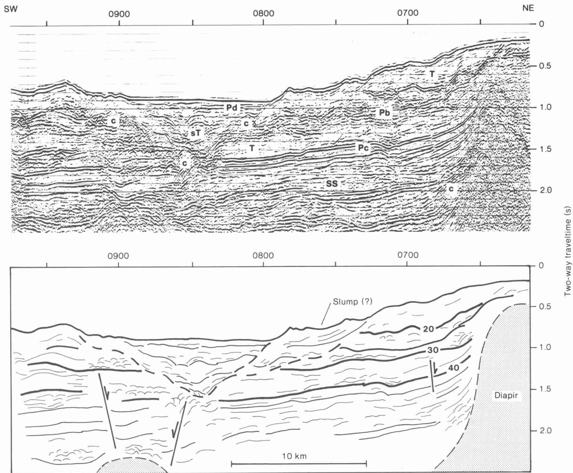
Figure 5. Multifold seismic profile and line drawing over continental slope showing Mississippi Canyon (dashed in line drawing) and interaction between sedimentation and diapirism (Line MC-27). See Figure 4 for location, Table 1 for seismic facies symbols, and Bouma, Coleman and Meyer (this volume) for discussion of the major seismic Horizons 20, 30, and 40.
