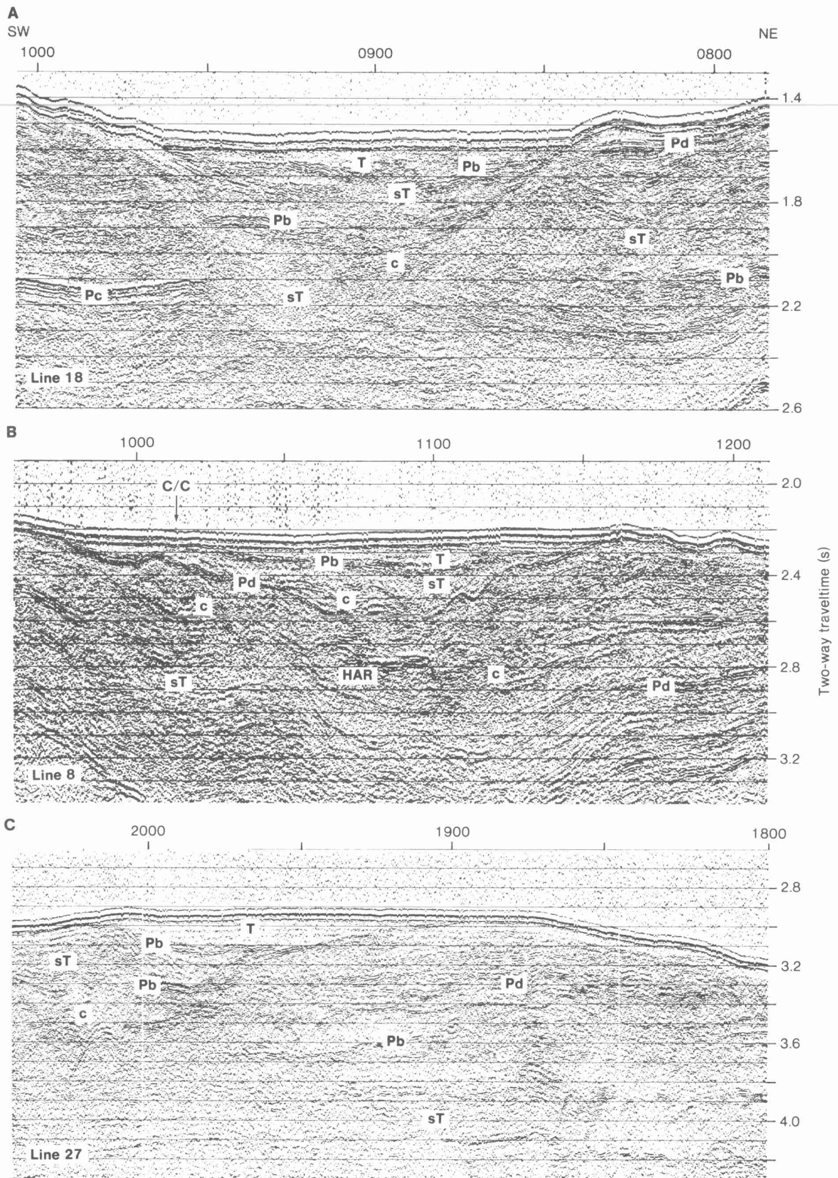
Figure 7. High-resolution (80 cu. in. water gun) seismic profiles and corresponding line drawings showing characteristics of upper fan channel (dashed in line drawings). Lines (R/V Conrad ) identified on seismic profiles. See Figure 4 for location; Table 1 for seismic facies symbols. C/C = course change.
