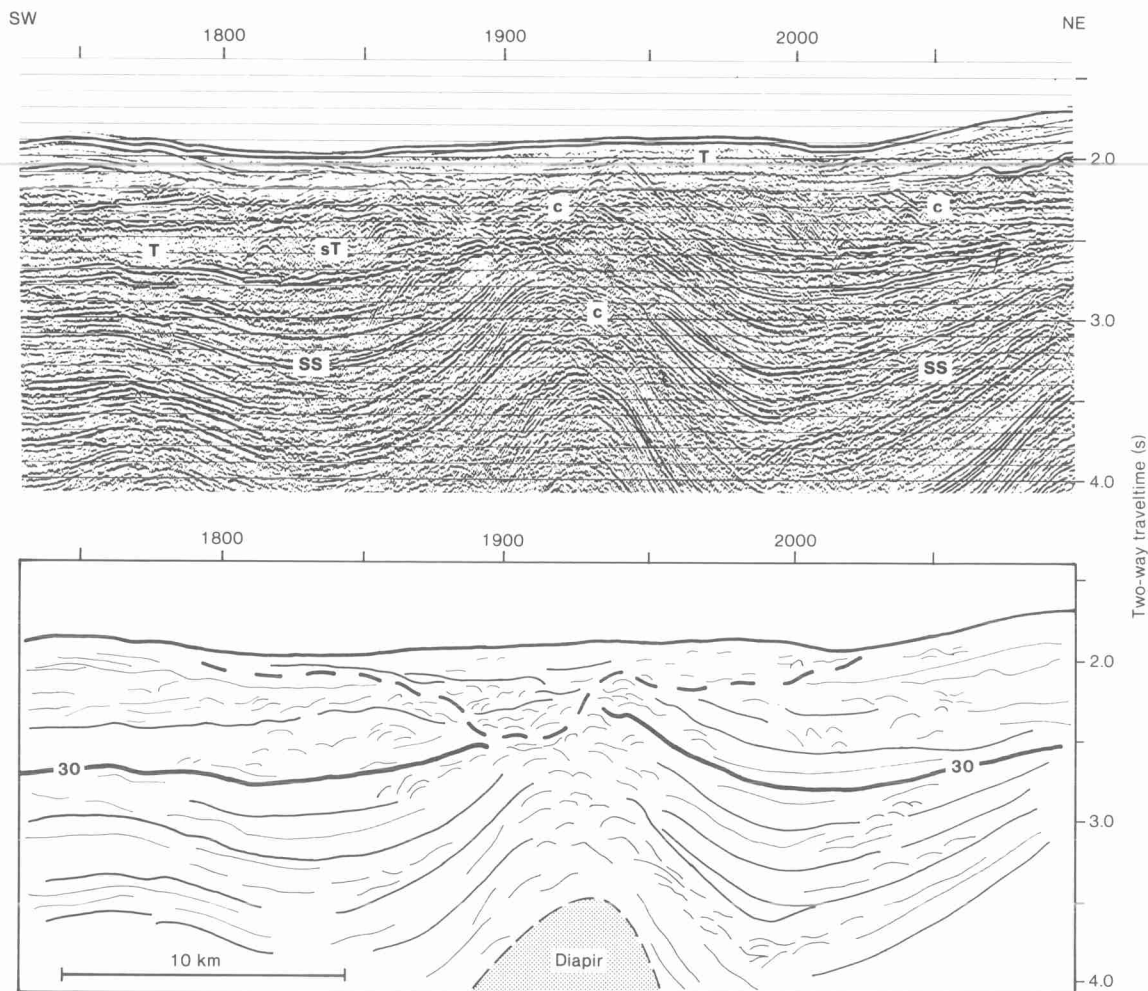
Figure 6. Multifold seismic profile and line drawing across upper fan showing modern channel (dashed in line drawing), intraslope-basin-type seismic sequences, and salt tectonics (Line MC-14). See Figure 4 for location; Table 1 for seismic facies symbols.
