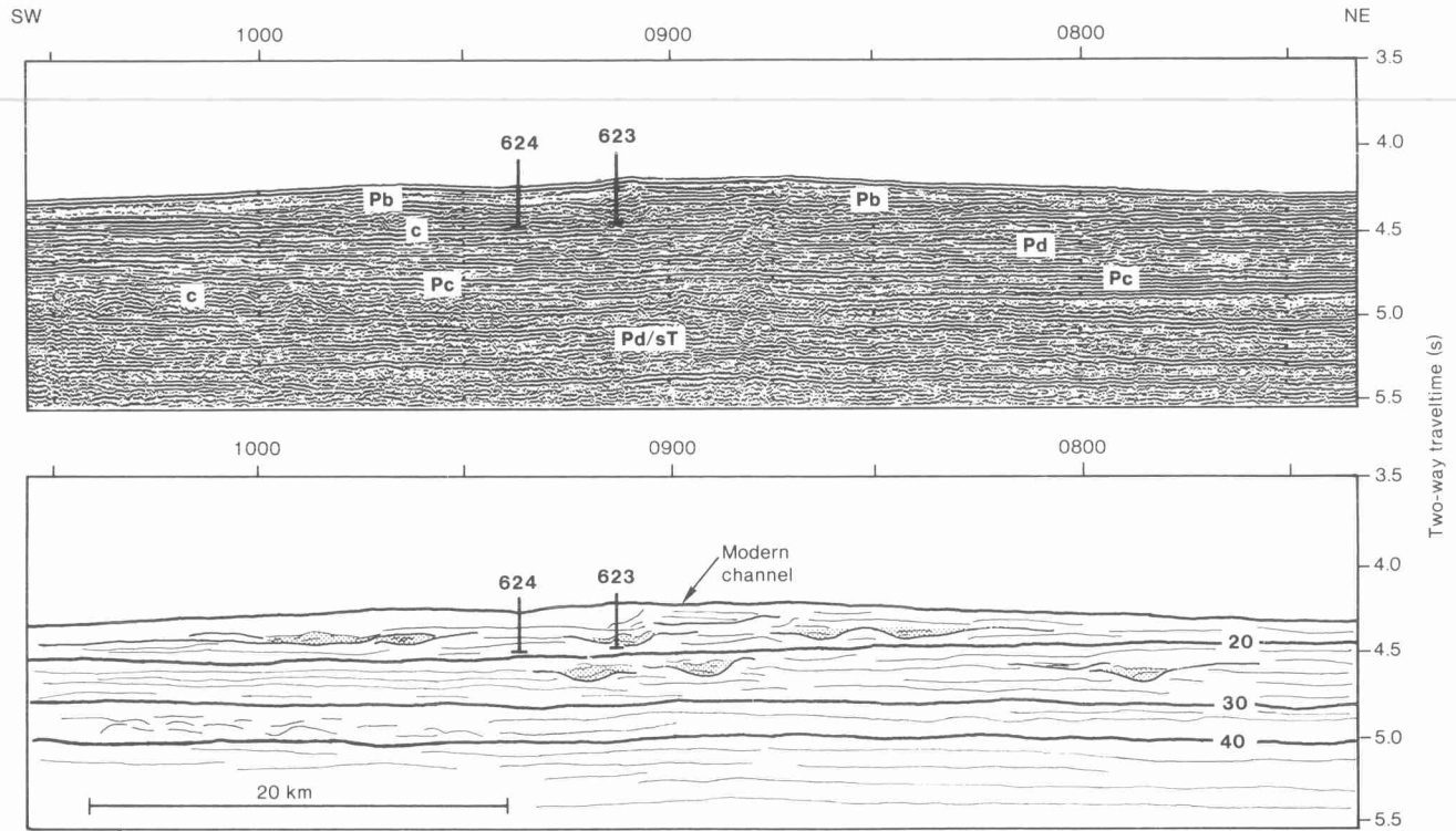
Figure 10. Sparker (160 kJ) seismic profile and line drawing over upfan region of the lower fan, showing inferred channels in Wisconsin fan lobes (U.S.N.S. Kane , Line KD-27). Relative positions of Sites 623 and 624 projected onto profile and drawing. See Figure 4 for location; Table 1 for seismic facies symbols.
