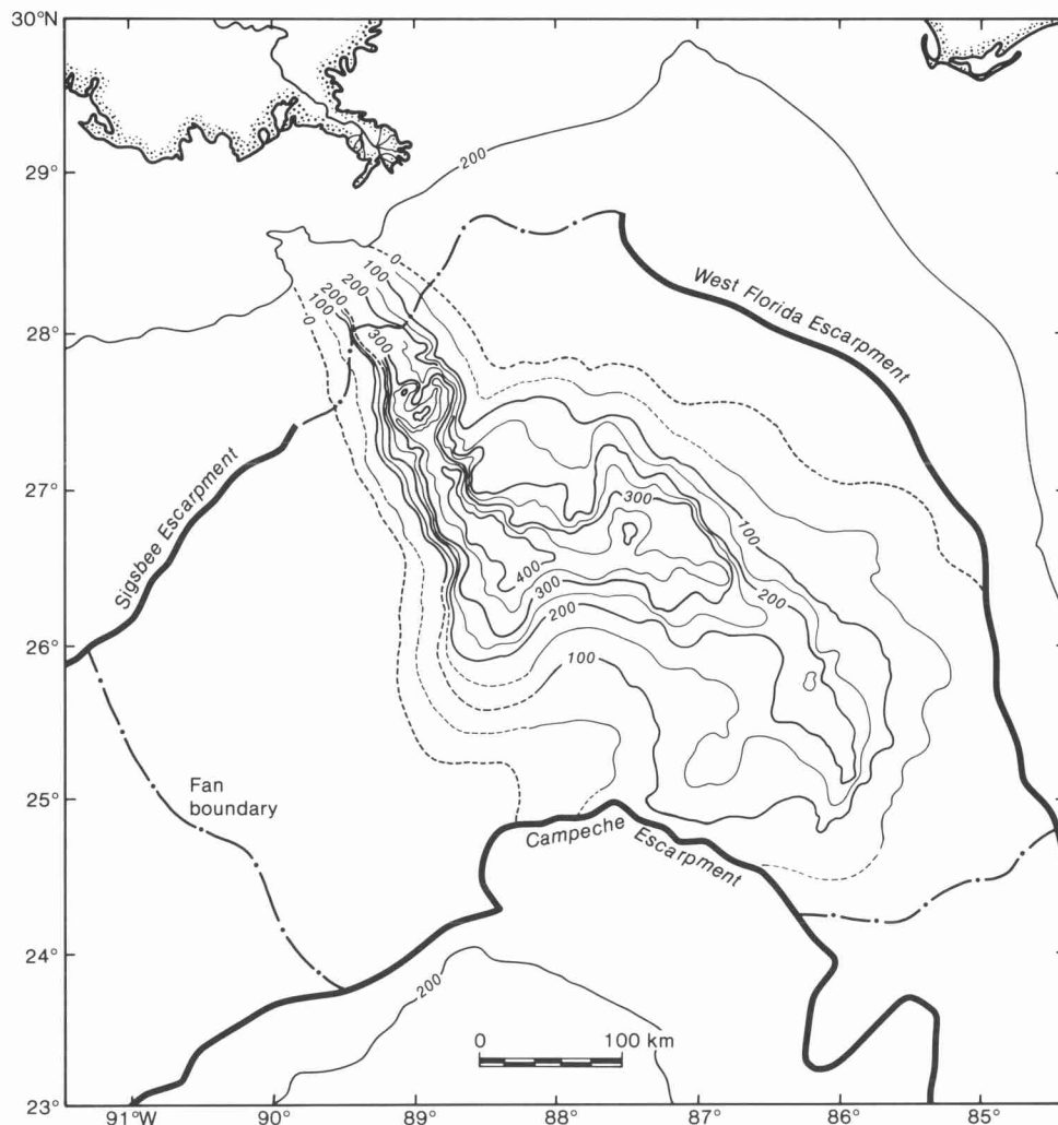
Figure 2. Isopach map of the youngest Mississippi Fan lobe. Maximum accumulations coincide with the channel complex. Isopach contours in meters. Modified after Bouma et al. (1983/84). Dashed line denotes either insufficient data or shallowing of reflector at seafloor. The 200-m isobath corresponds to shelf break.
