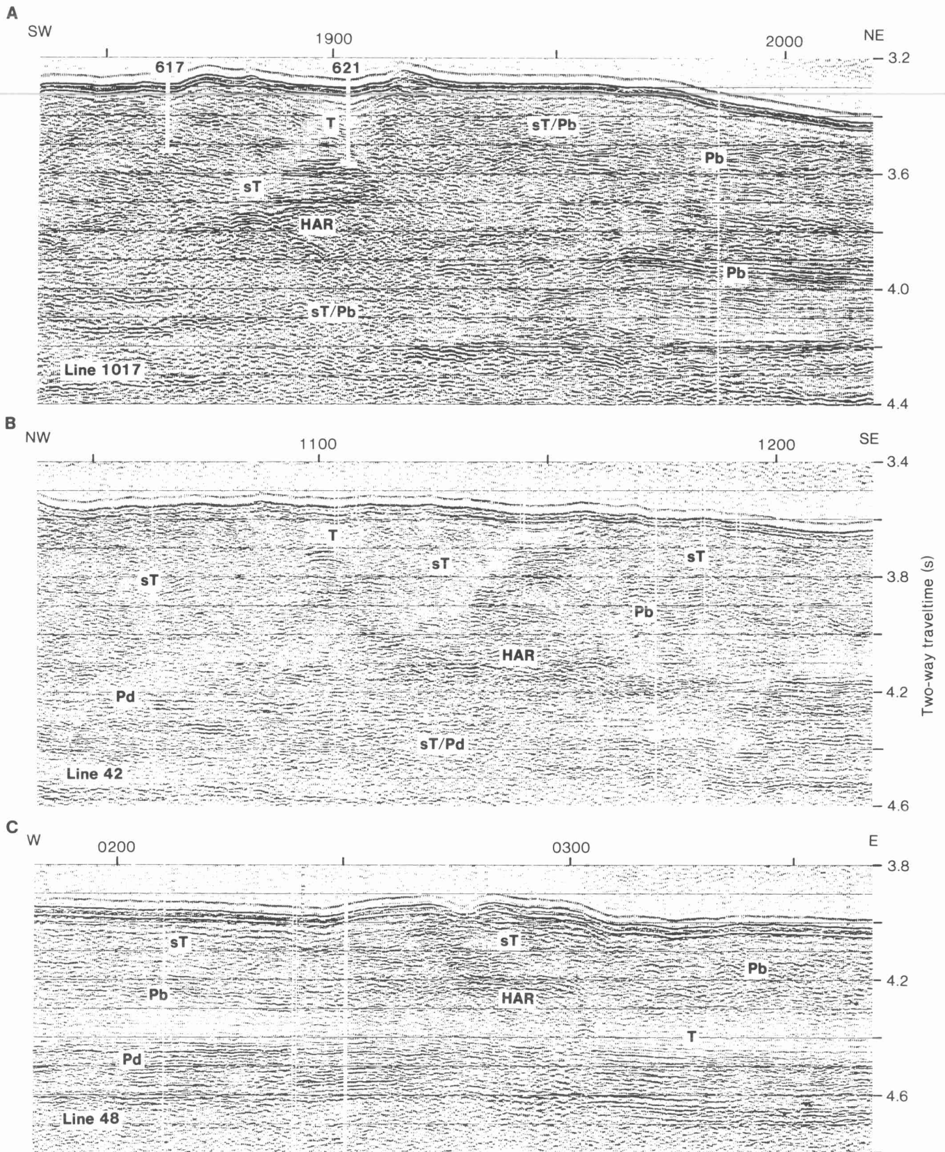
Figure 9. High-resolution (80 cu. in. water gun) seismic profiles and corresponding line drawings showing characteristics of middle-fan channel and location of Sites 617 and 621 (Fig. 9A). Lines (R/V Conrad ) identified on seismic profiles. For a discussion of thalweg deposits in channel complex see text. See Figure 4 for location; Table 1 for seismic facies symbols.
