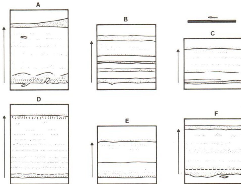
Fig. 4. Six characteristic sedimentation units in recent Scotian margin turbidites (shown by arrows). Sketch sections from microscopic/X-radiographic core study.
